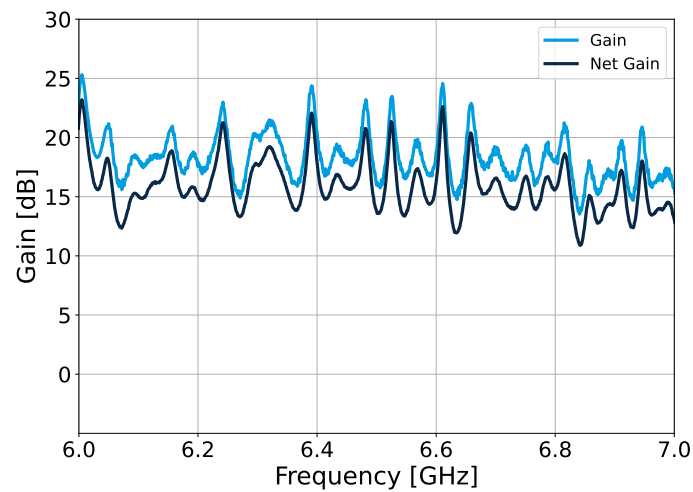
Figure 4: Zoom on the gain (ON-OFF) and net gain (ON-lossless reference) of the TWPA. The pump parameters are (at the input of the TWPA): 5.540 GHz and -66.5 dBm.
