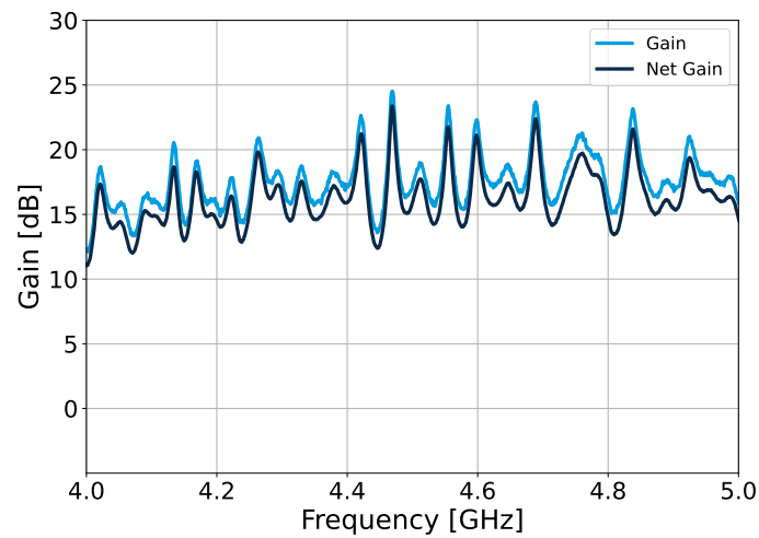
Figure 3: Zoom on the gain (ON-OFF) and net gain (ON-lossless reference) of the TWPA. The pump parameters are (at the input of the TWPA): 5.540 GHz and -66.5 dBm.
