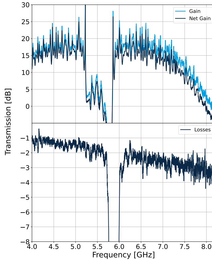
Figure 2: Top panel shows the gain (ON-OFF) and net gain (ON-lossless reference) of the TWPA. The pump parameters are (at the input of the TWPA): 5.540 GHz and -66.5 dBm. Bottom panel shows the electrical losses within the TWPA. The gap is centered at 5.89 GHz and is 0.34 GHz wide, the signal cannot propagate in the gap.
